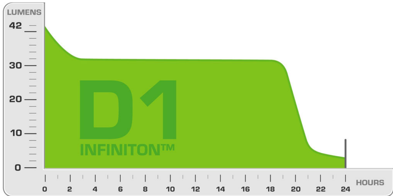
Light intensity over time Lightwave™ Infiniton™ D1
